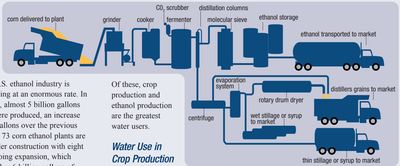
Dry grind corn ethanol production process (modified from Renewable Fuels Association, 2007)
